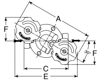
Series TVS 811/812/813 - Top View
